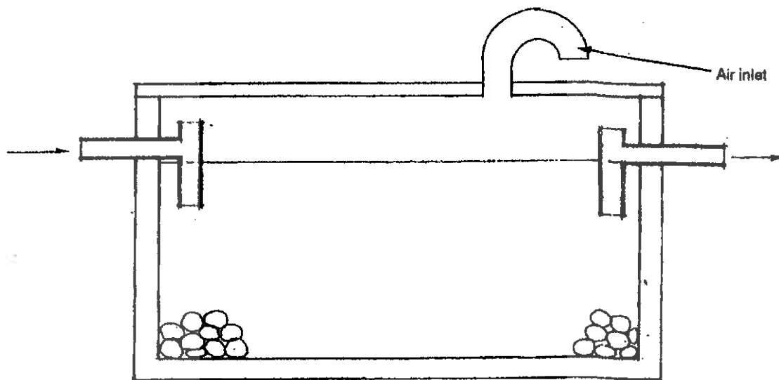
FIGURE 3.5 AEROBIC FILTER
