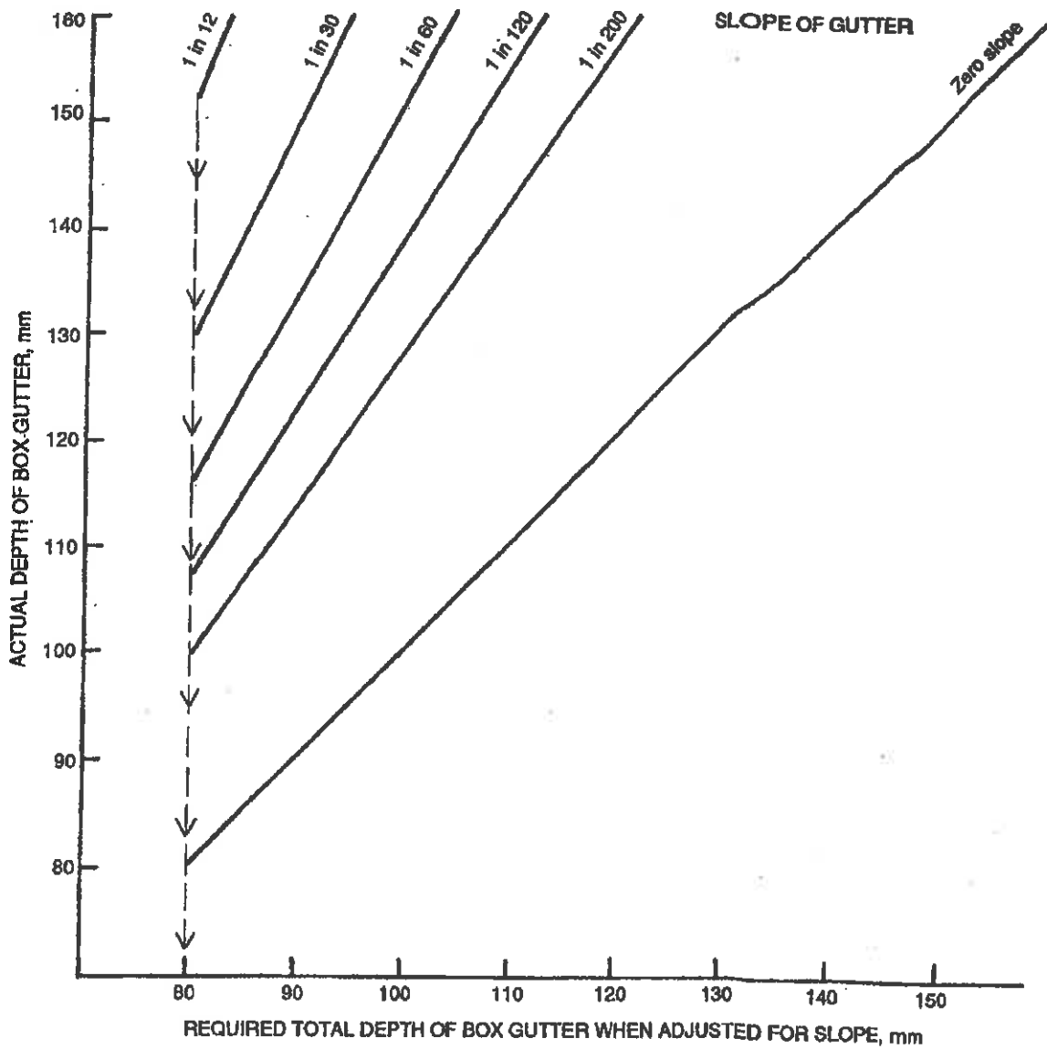
FIGURE 4.1.3 BOX GUTTER DEPTH - ADJUSTED FOR SLOPE
