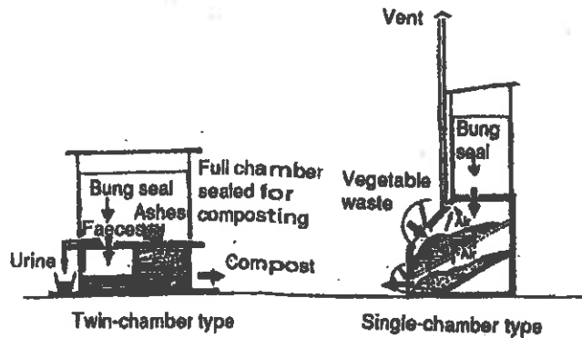
FIGURE 4.1 COMPOSTING LATRINES
