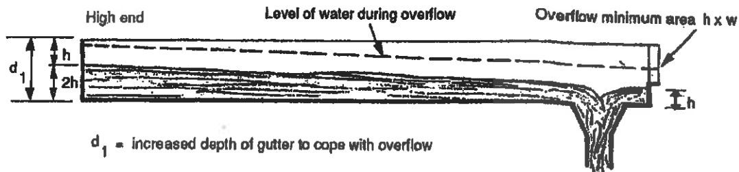
FIGURE 4.3.2 OVERFLOW WITH BLOCKED DOWNPIPE
