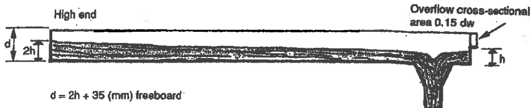
FIGURE 4.3.1 OVERFLOW OUTLET
