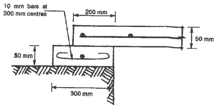
FIGURE 4.3A DETAILS OF SQUAT TYPE COVER SLAB
