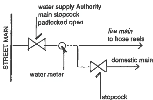
FIGURE 2 WATER SUPPLY RETICULATION: COMBINED SERVICES
