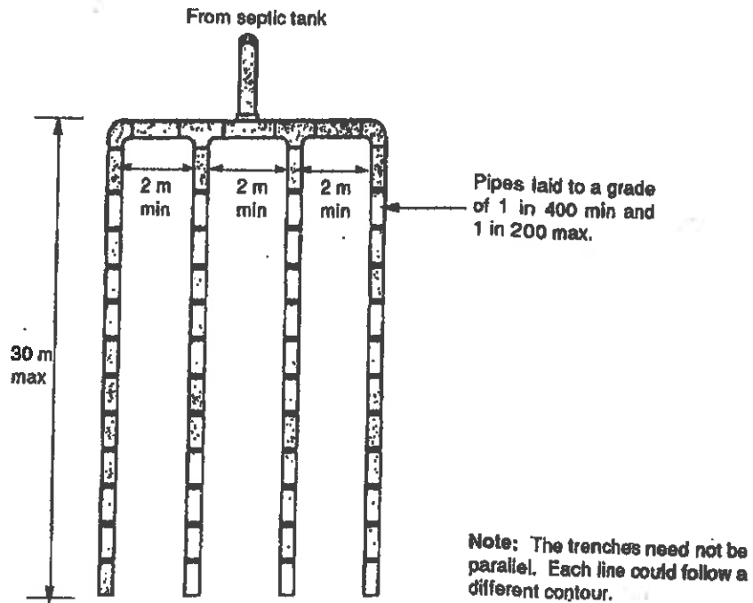
FIGURE 6.4B GENERAL LAYOUT OF ABSORPTION TRENCH
