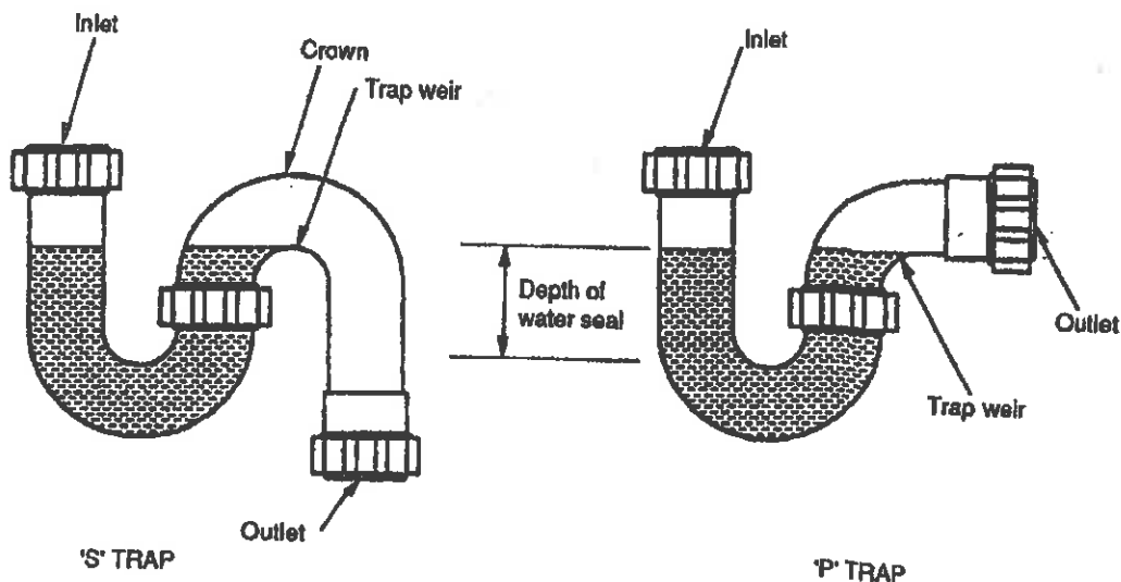
FIGURE DF6.1.2 EXAMPLES OF FIXTURE TRAPS
