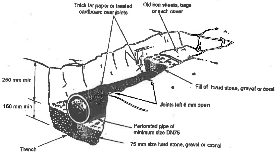
FIGURE 6.4A EXAMPLE OF AN ABSORPTION TRENCH
