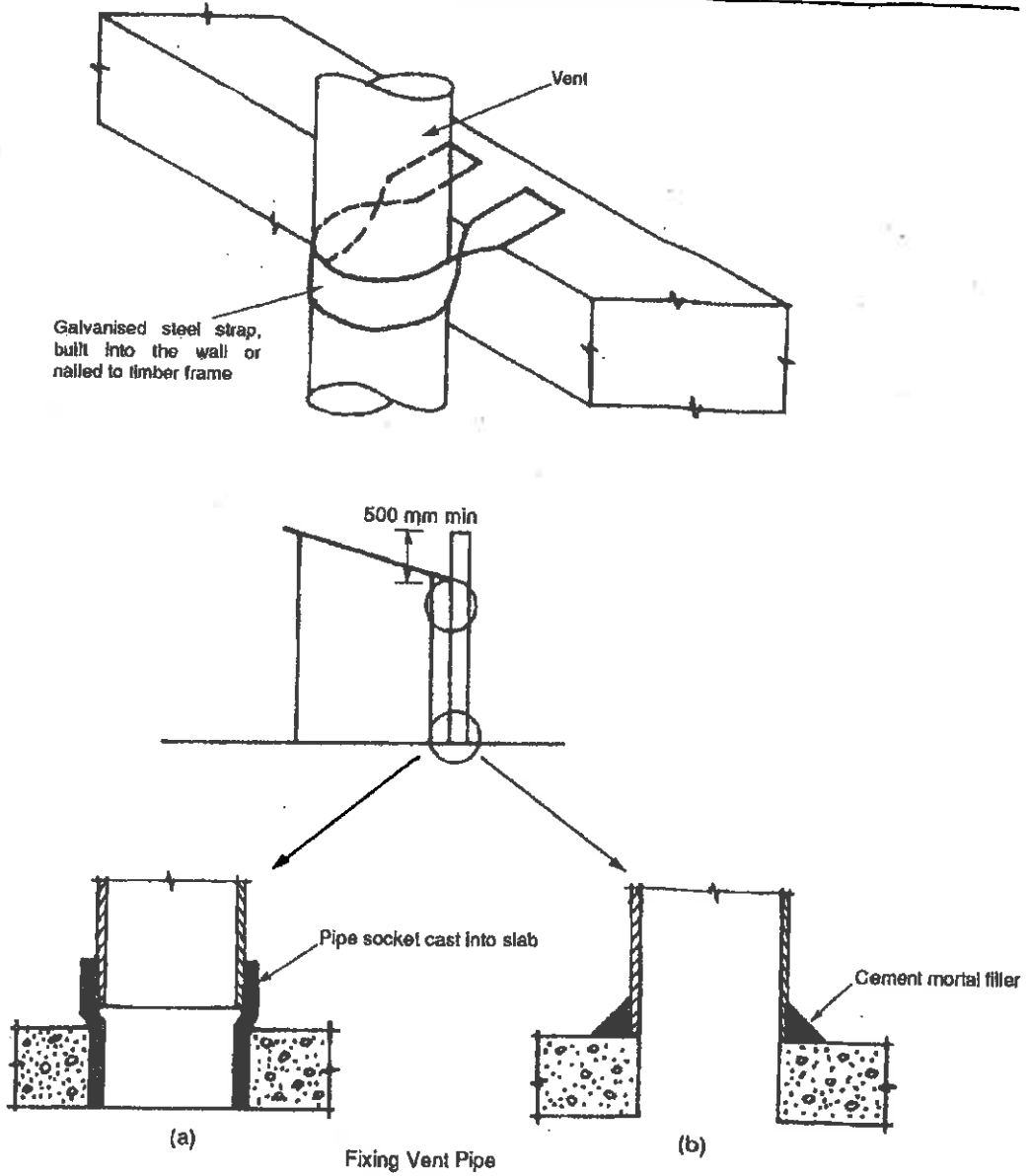
FIGURE 4.4A METHODS OF FIXING THE VENT PIPE
