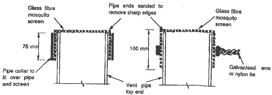
FIGURE 4.4B FIXING OF INSECT SCREEN OVER VENT PIPE
