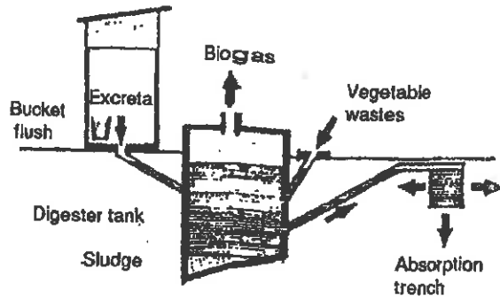
FIGURE 4.6 BIOGAS DIGESTER
