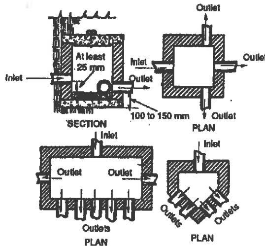
FIGURE 8.1 EXAMPLES OF DISTRIBUTION BOXES
