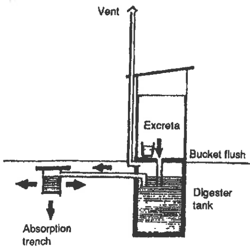
FIGURE 4.4 AQUA PRIVY
