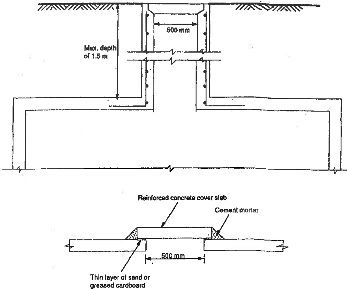
FIGURE 3.4C TWO ALTERNATIVE METHODS OF PROVIDING MANHOLE COVERS
