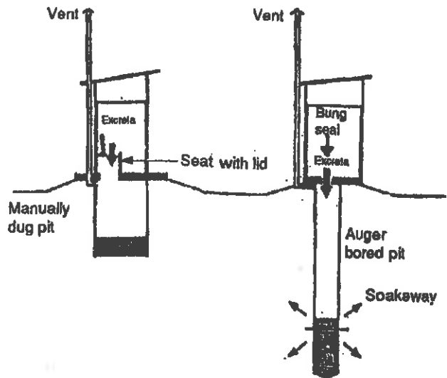
FIGURE 4.2 DRY (NONFLUSH) PIT LATRINES
