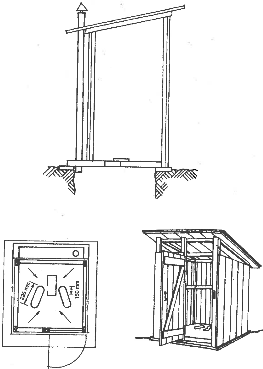
FIGURE 4.5 GENERAL ARRANGEMENT
