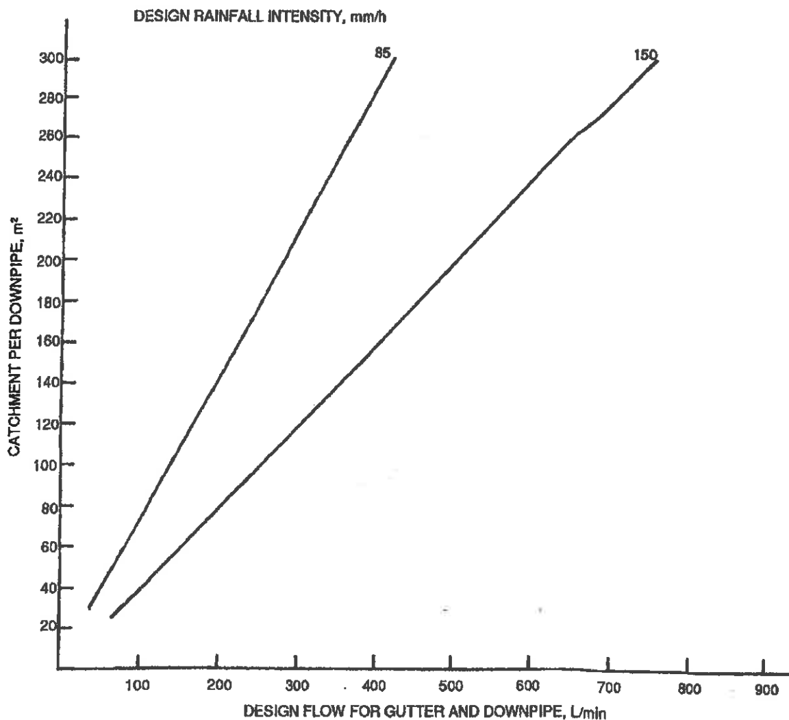
FIGURE 4.1.1 INTERNAL BOX GUTTER DESIGN FLOW
